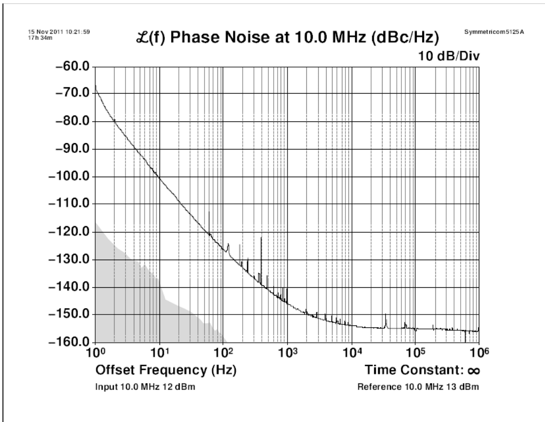
Figure 3.14 Typical LC-XO-Plus Phase Noise
