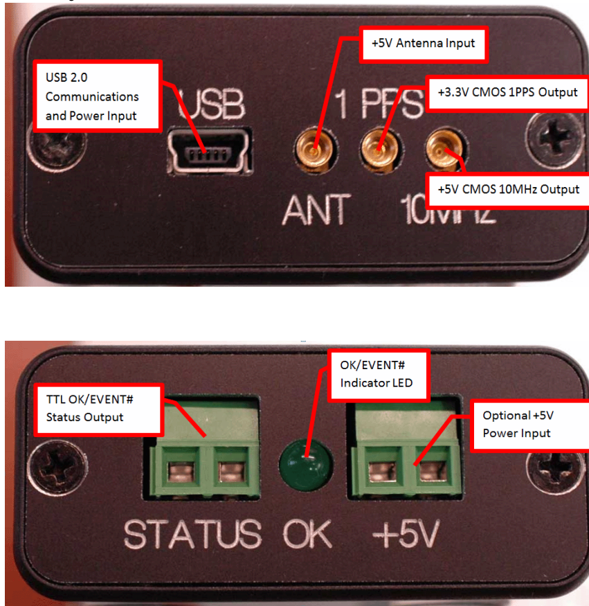
Figure 2.3 Major connections to LC-XO-PLUS enclosure
