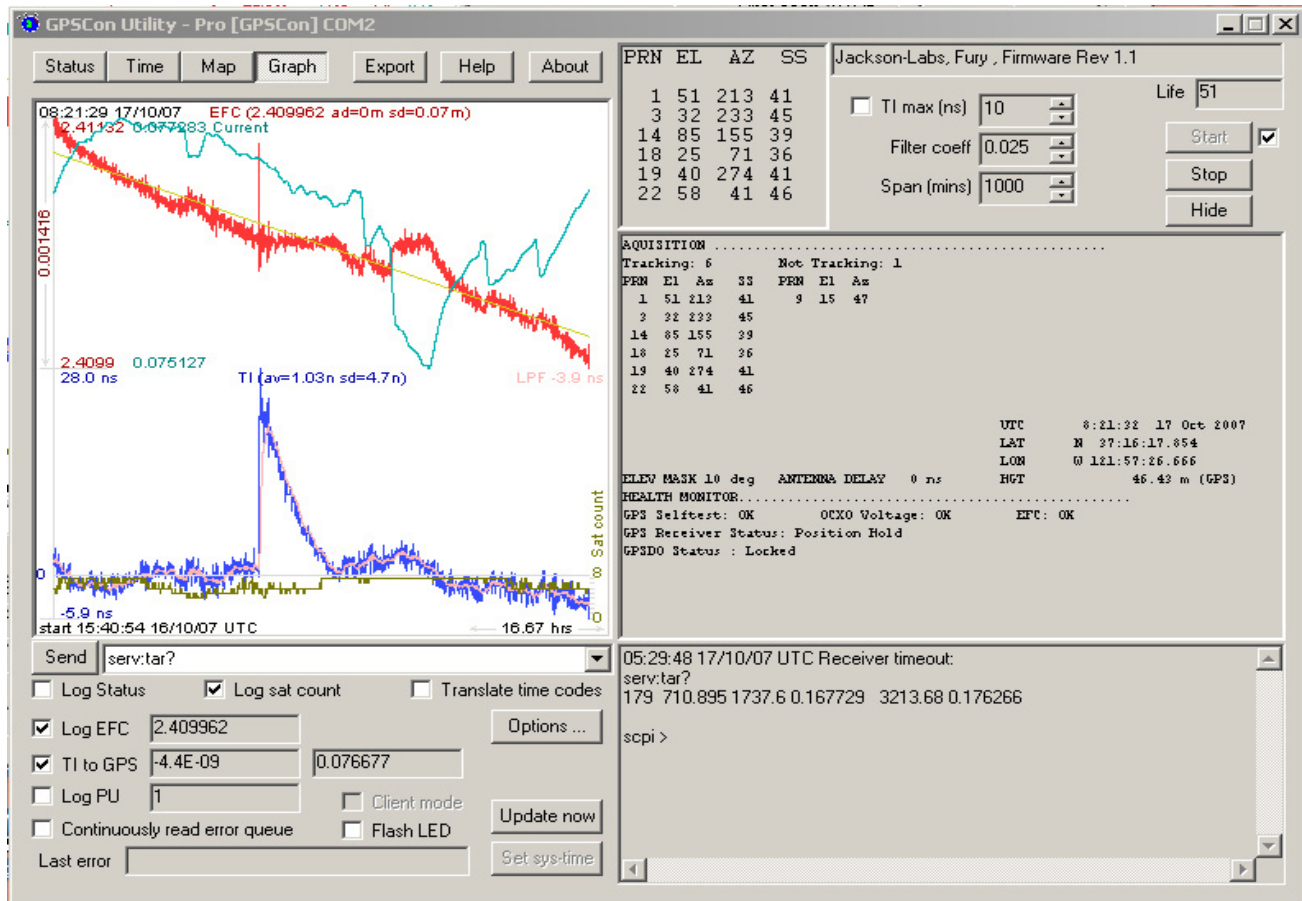
Figure 2.4 LC-XO-PLUS GPSDO phase compensation plo
